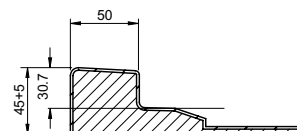
Tray Profile
